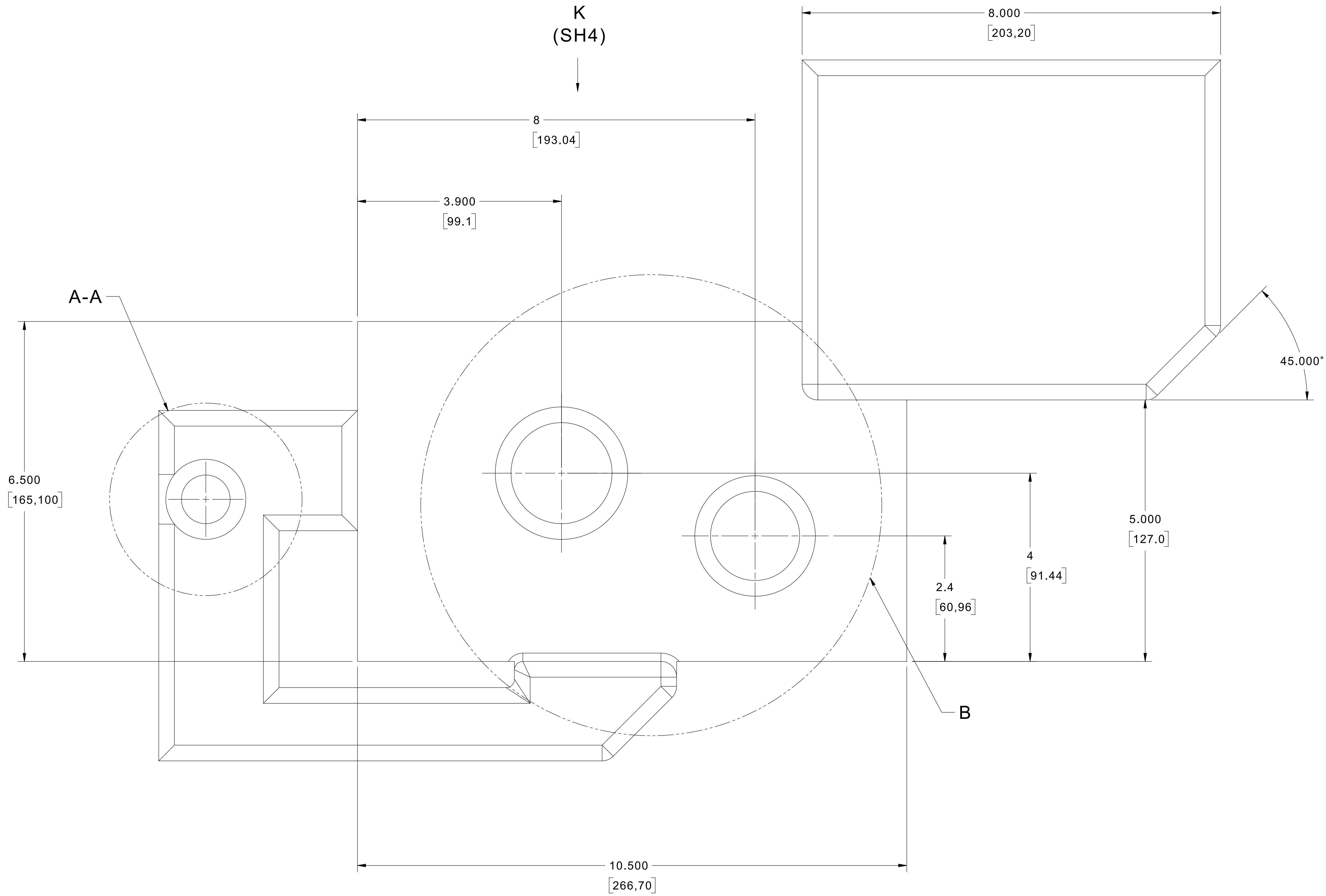
TOP VIEW
