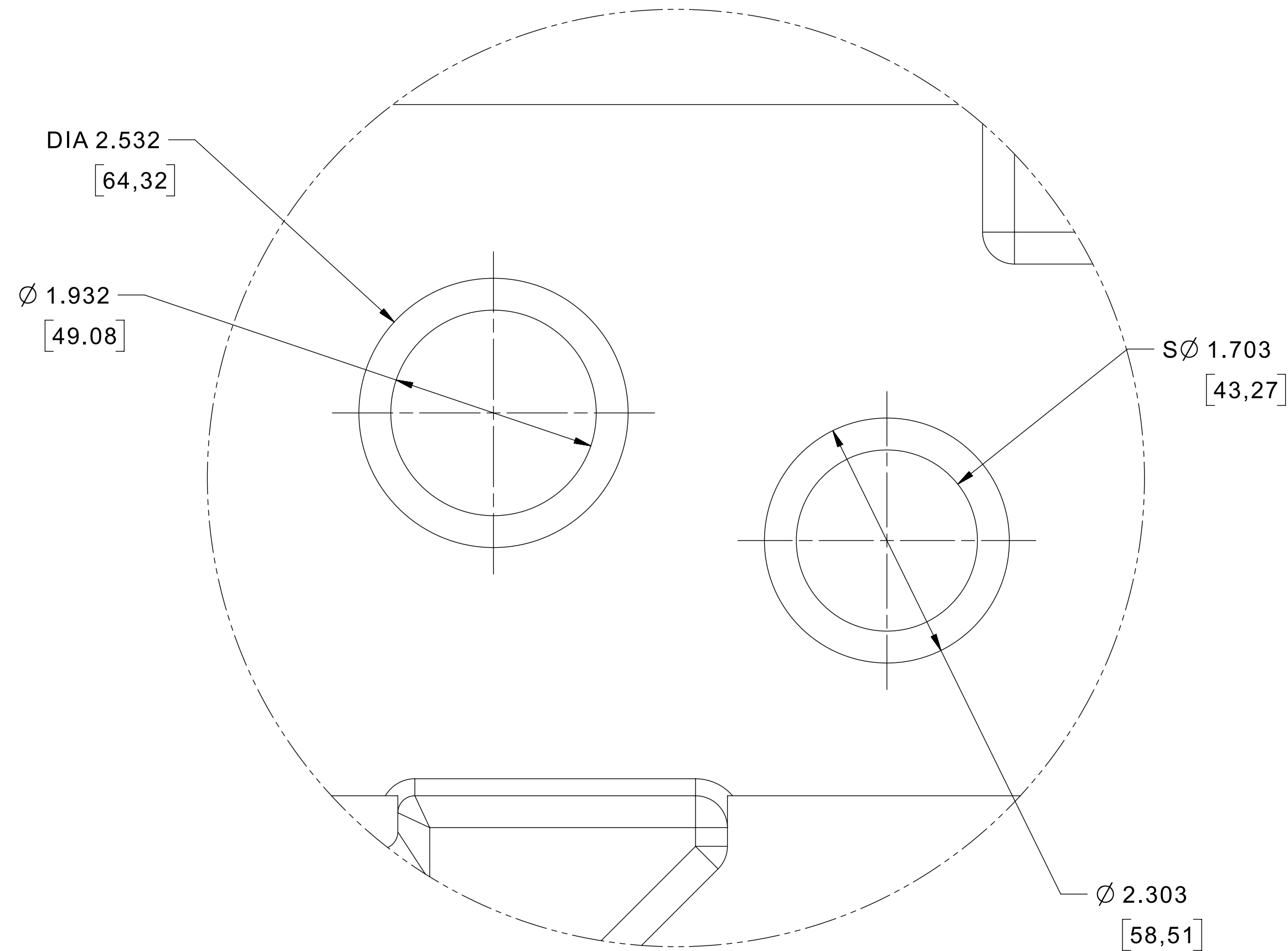
DETAIL B(H12,SH3)
