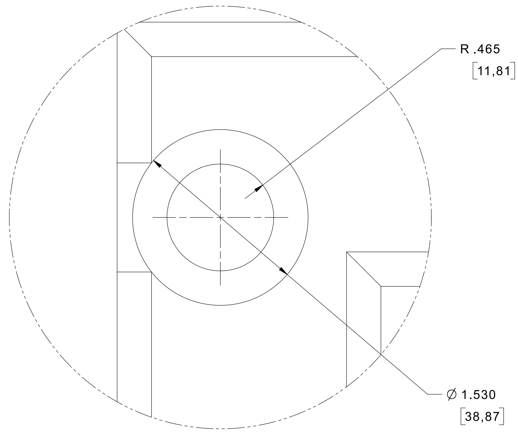
DETAIL A-A (F8,SH2)
